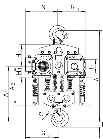
Model CPE/CPEF 100-2 with suspension hook, 10000 kg
